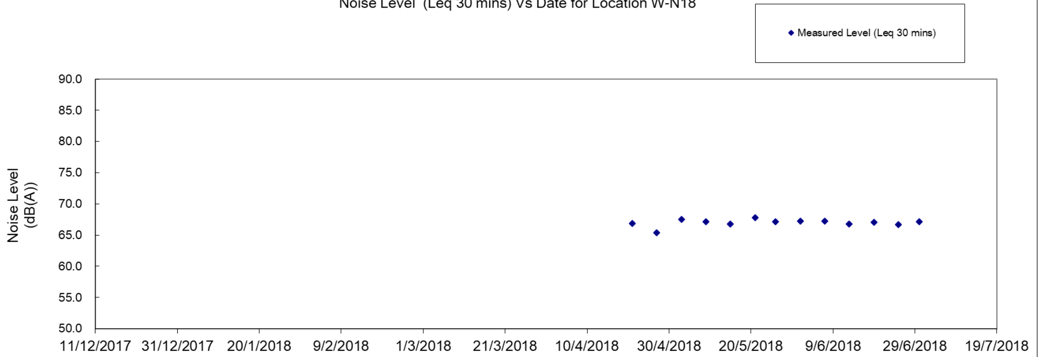
Noise Level (Leq 30 mins) Vs Date for Location W-N18
